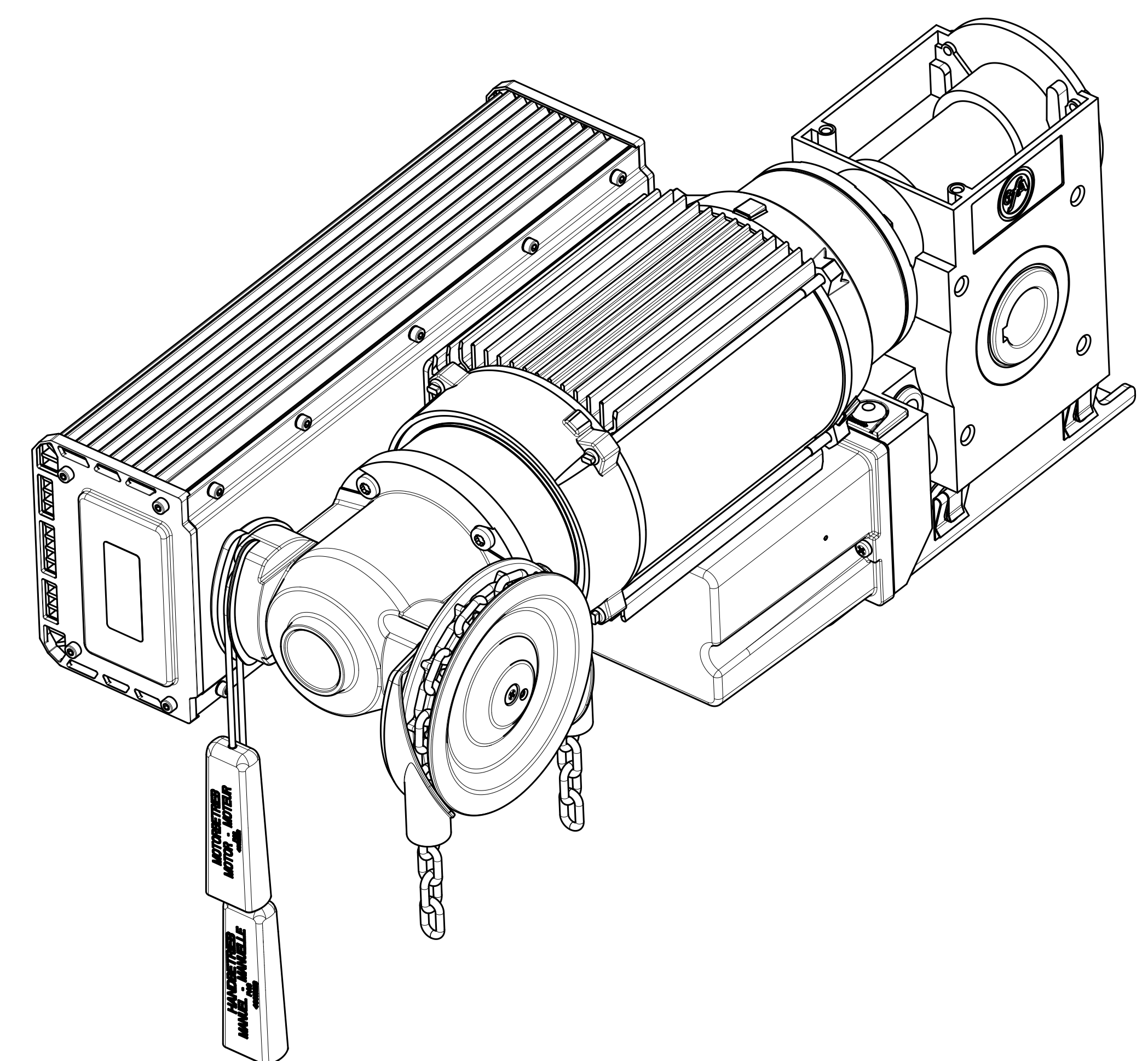
Darstellung: Einbaulage FU links illustration: FI on the left side
