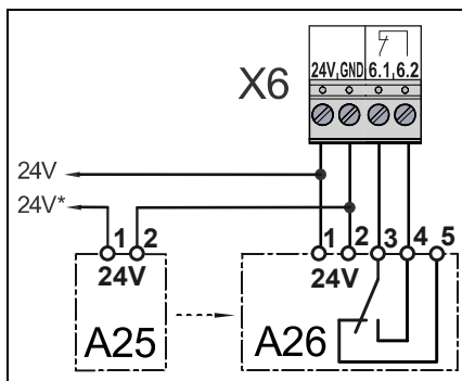
Light curtain A25: Transmitter A26: Receiver
