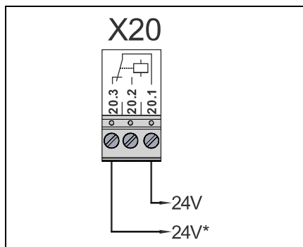
X20: Function relay (Test light curtain)
