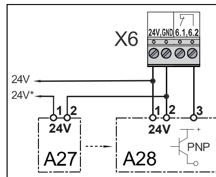
Light curtain A27: Transmitter A28: Receiver
