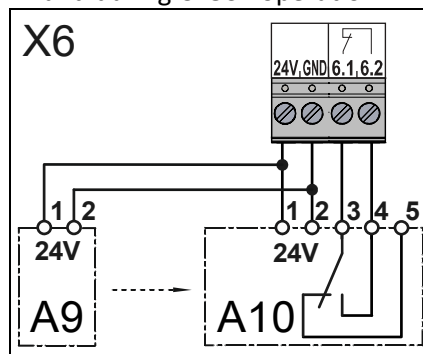
Through photocell A9: Transmitter A10: Receiver
